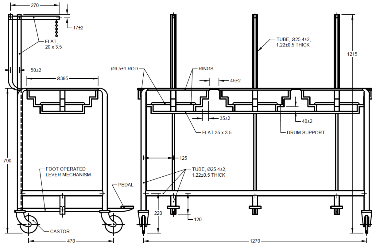
Fig. 1 DRESSING DRUM TROLLEY
